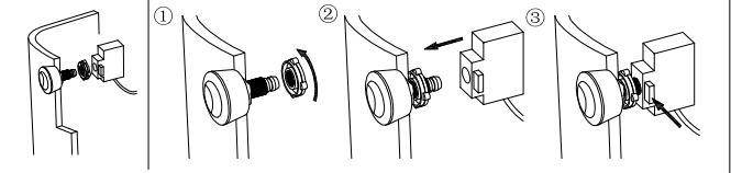
Installation of the side push button -2
