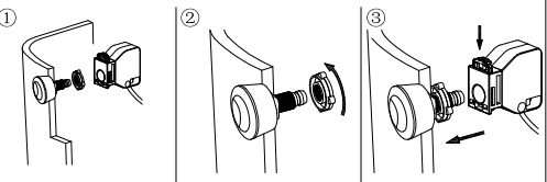
Installation of the side push button -2
