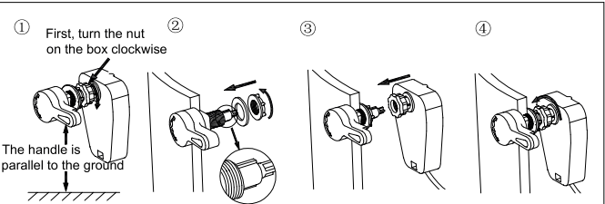
Installation of the side push button -1
